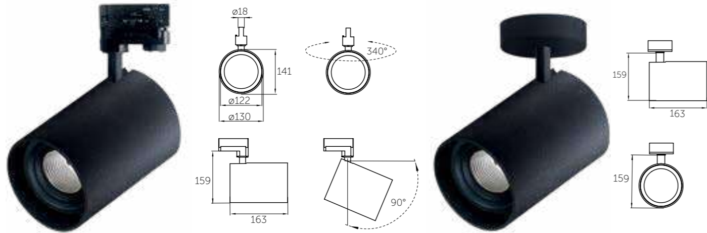
TRACK A RIEL
